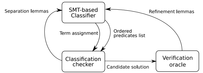
Fig. 1: Unif+PI loop.
